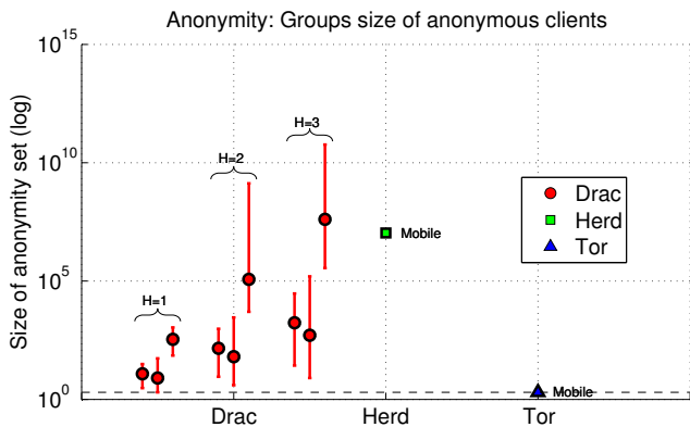
Figure 4: Size of anonymity sets for Drac , Herd , and Tor : median, 10th, and 90th percentiles (left to right). For Drac , we show the results for the Mobile , Twitter , and Facebook datasets and H = 1, 2, 3 , and for Tor , the results for the Mobile dataset. The size of anonymity sets in Herd is independent of the node degree and workload.
