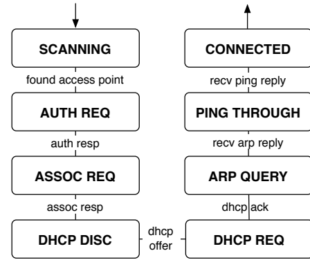
Figure 5: Steps involved in connection establishment. Establishing a connection requires a minimum of 13 frames.
